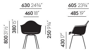
Eames Plastic Armchair DAX, four-legged tubular steel base, with full upholstery
