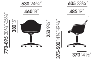
Eames Plastic Armchair PACC, castor-based swivel chair, with full upholstery
